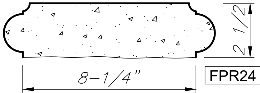
DOUBLE BULLNOSE FIREPIT COPING
